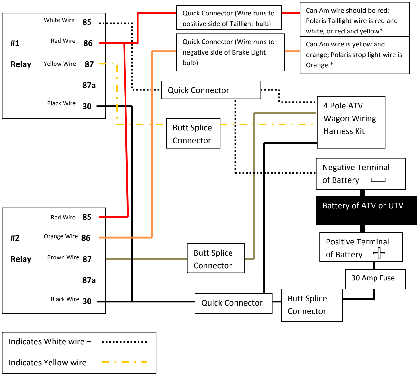
Positive Ground Relay System
